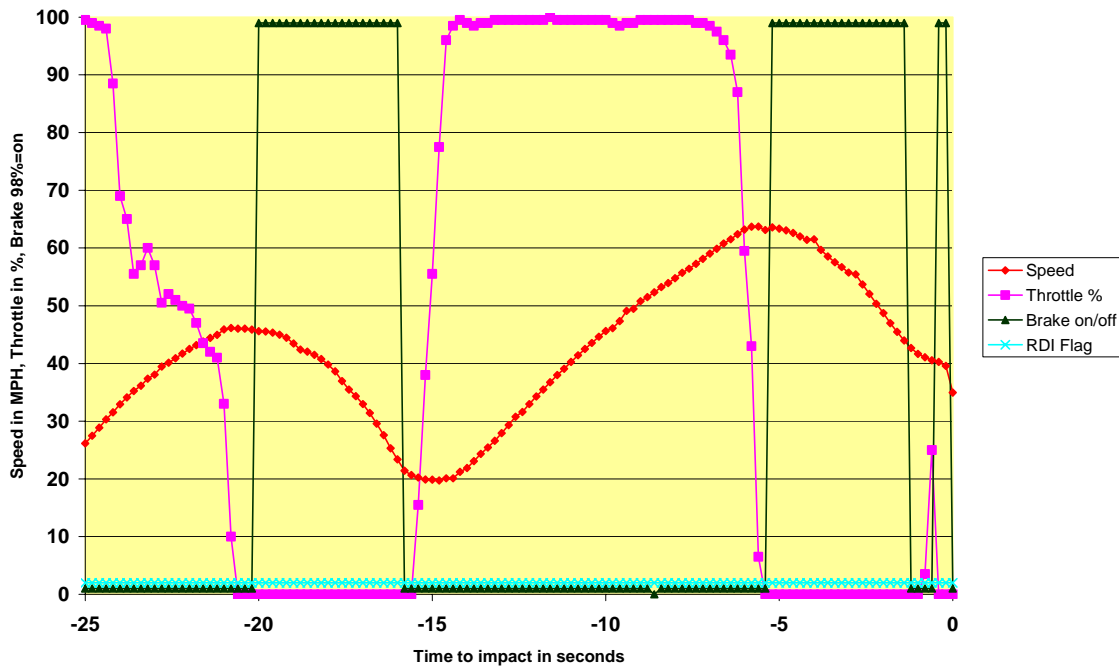
Example Ford PCM Event Data Recorder with Power Loss at Impact
